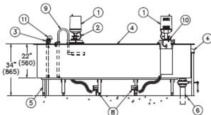
STATIONARY F-425-S IMMERSION TANK
