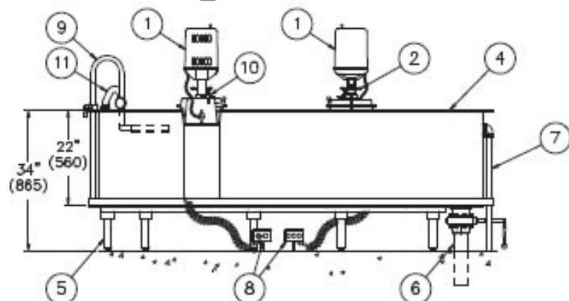
STATIONARY F-270-S IMMERSION TANK
